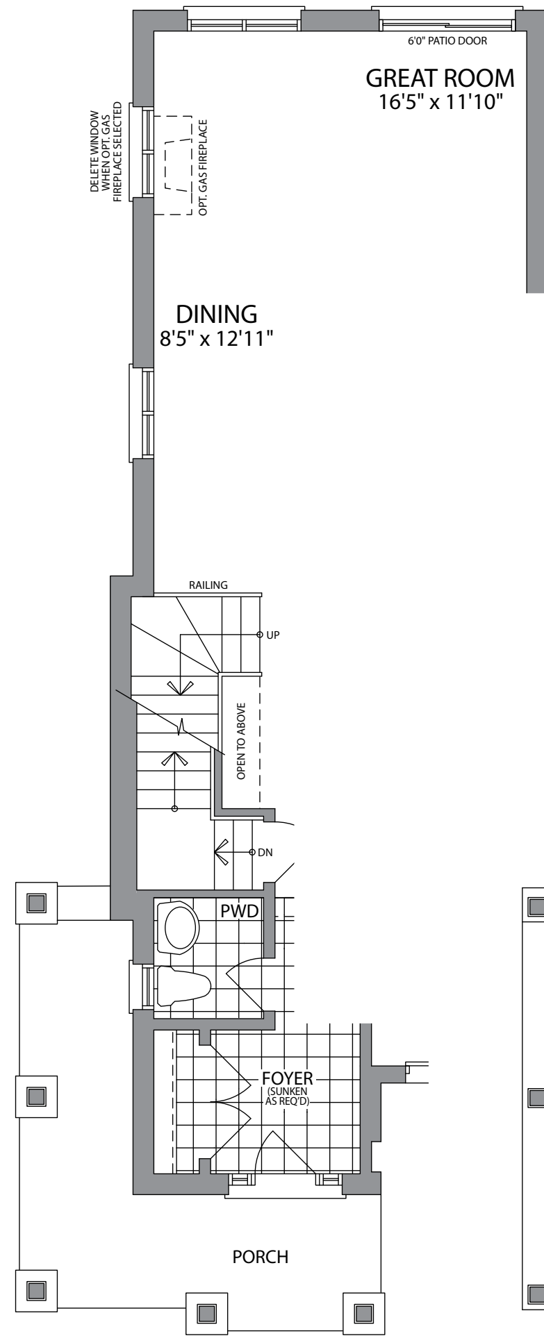
GROUND FLOOR ELEVATION B
