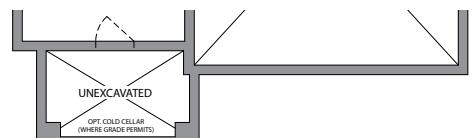
BASEMENT ELEVATION B
