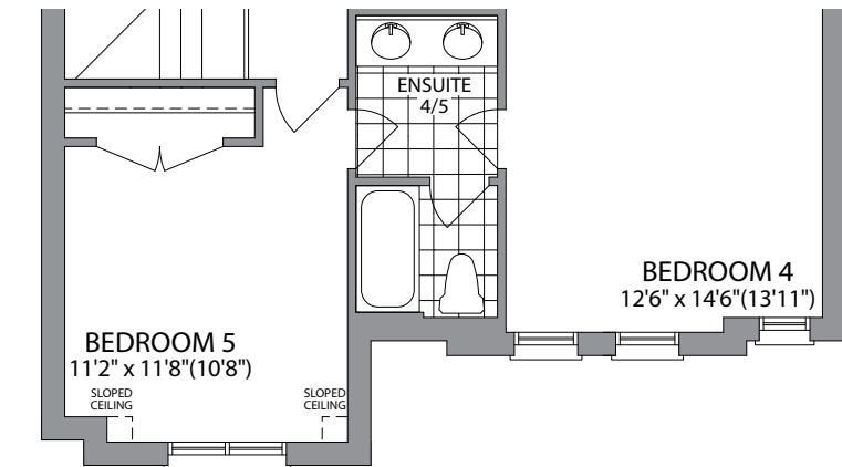
OPT. SECOND FLOOR ELEVATION B
