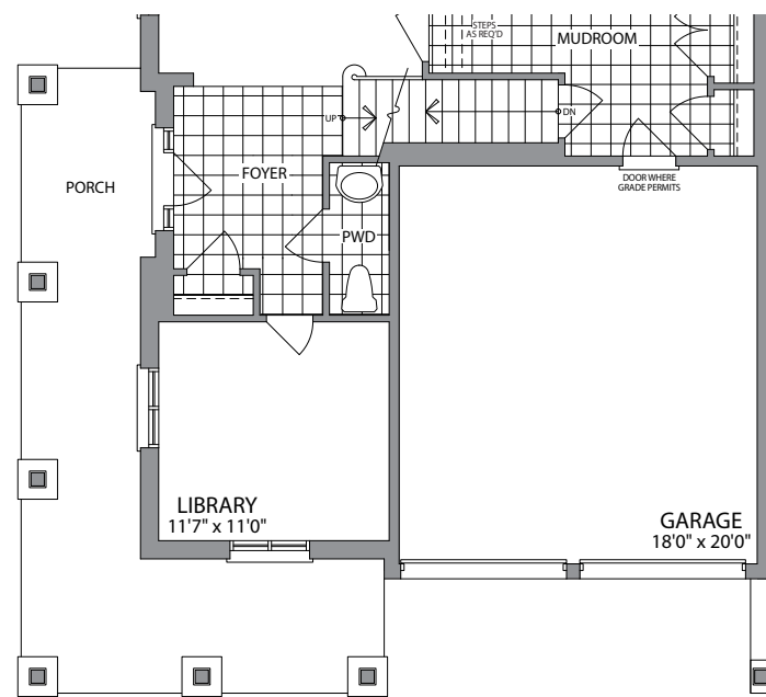
GROUND FLOOR ELEVATION B
